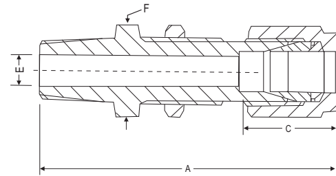
Dimensional Details :
